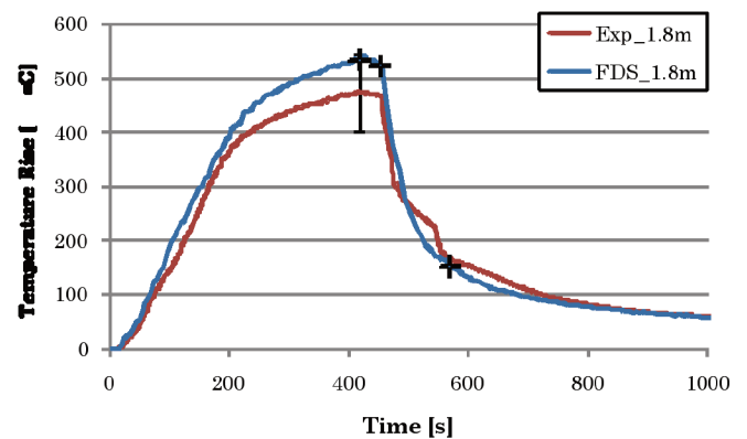
Figure 41: Measured vs. Predicted Temperature at the 1.8 m (5.9 ft) Thermocouple Location in the Burn Compartment
